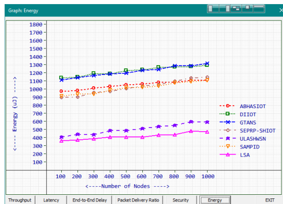
Figure 11: Energy (uJ)
