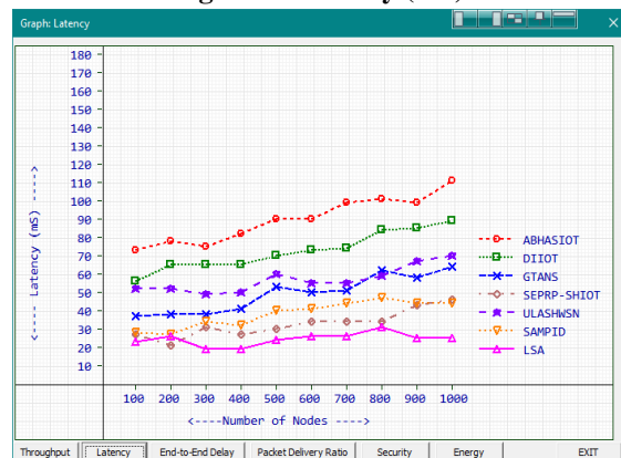
Figure 7: Latency (mS)
